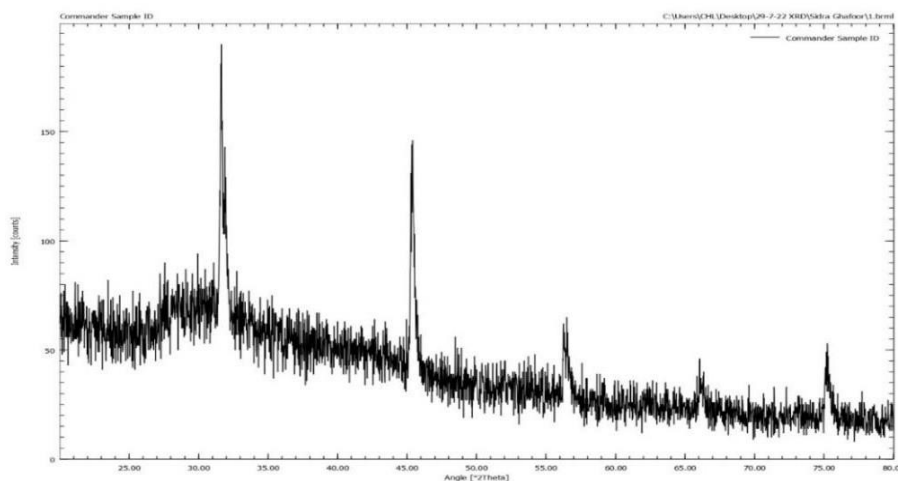
Figure 6. XRD of Starch-g-Polyacrylamide composite containing 1% \text{ZnSO}_4 salt. Five sharp peaks with high intensity show the strong interaction between composite and metal salt
