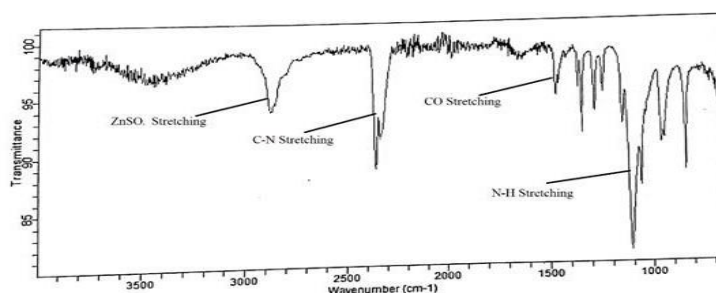
Figure 10. FTIR spectrum of composite containing 10 % ZnSO 4 .
