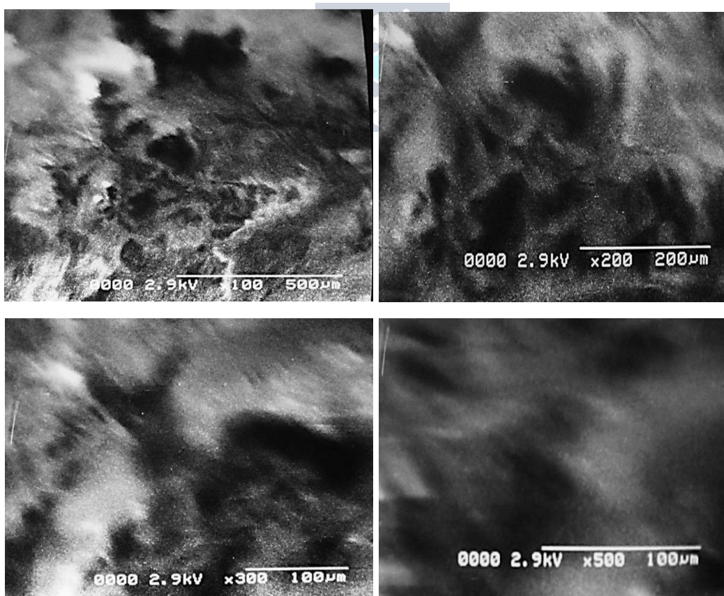
Figure 4. SEM images starch/polyacrylamide composite containing 1% ZnSO 4 having high extent of roughness than 10 % ZnSO 4 salt.
